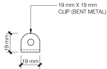
03 90 DEGREE CLIP FRONT ELEVATION 1:2 SCALE
