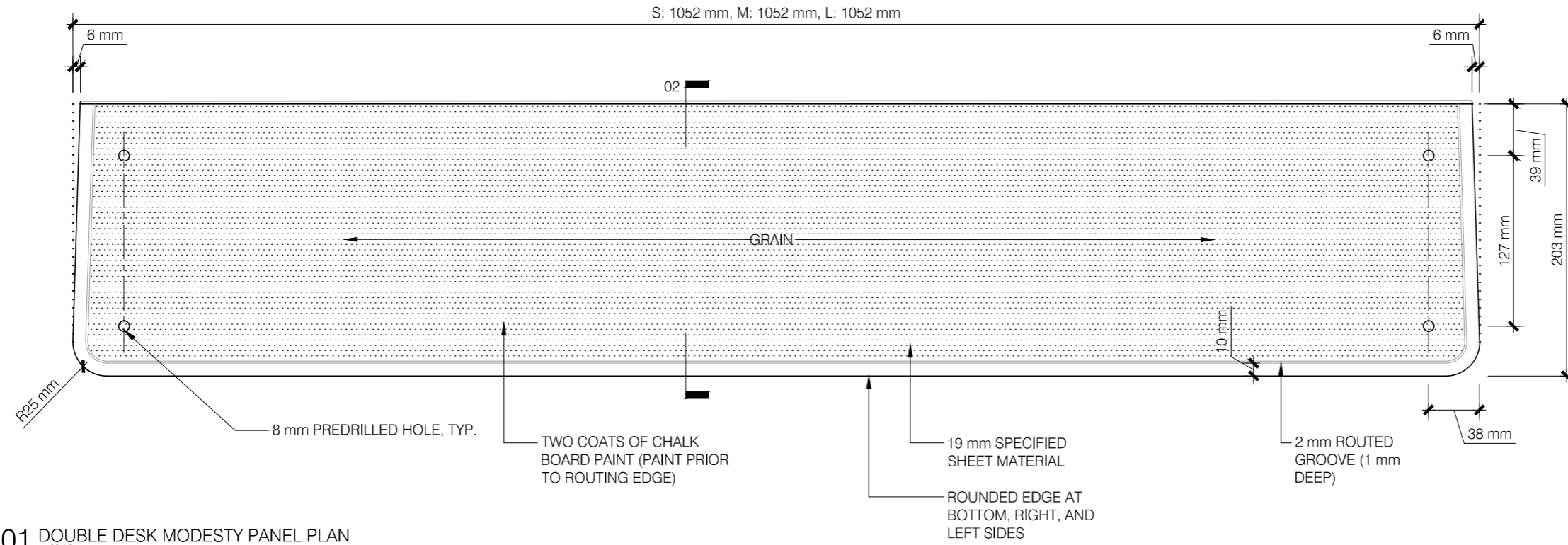
01 DOUBLE DESK MODESTY PANEL PLAN 1:4 SCALE
