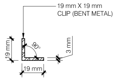
04 90 DEGREE CLIP SECTION 1:2 SCALE
