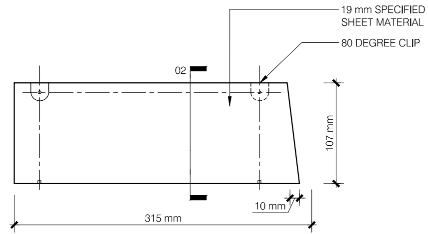
01 SHELF DIVIDER ELEVATION 1:4 SCALE
