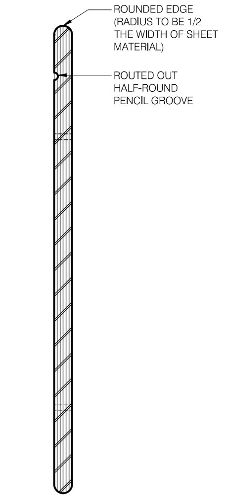
03 DESK TOP SECTION 1:4 SCALE
