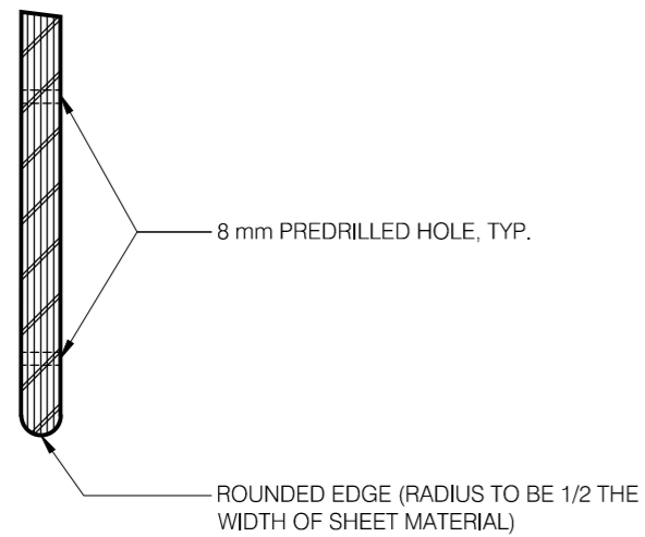
02 DOUBLE DESK MODESTY PANEL SECTION 1:4 SCALE
