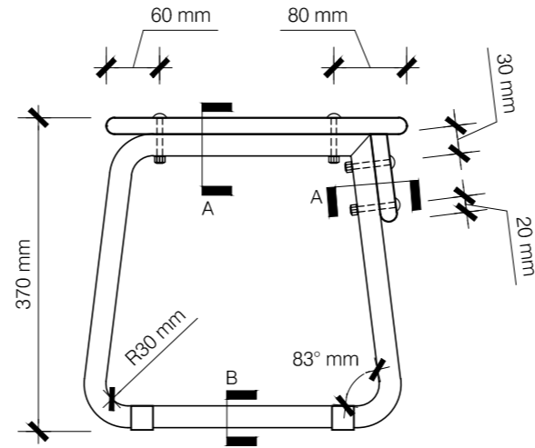
02 BENCH SIDE ELEVATION 1:8 SCALE
