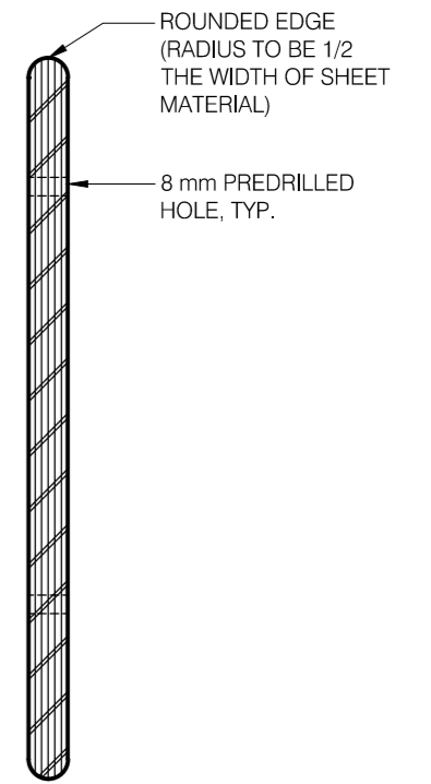
03 BENCH SEAT SECTION 1:4 SCALE
