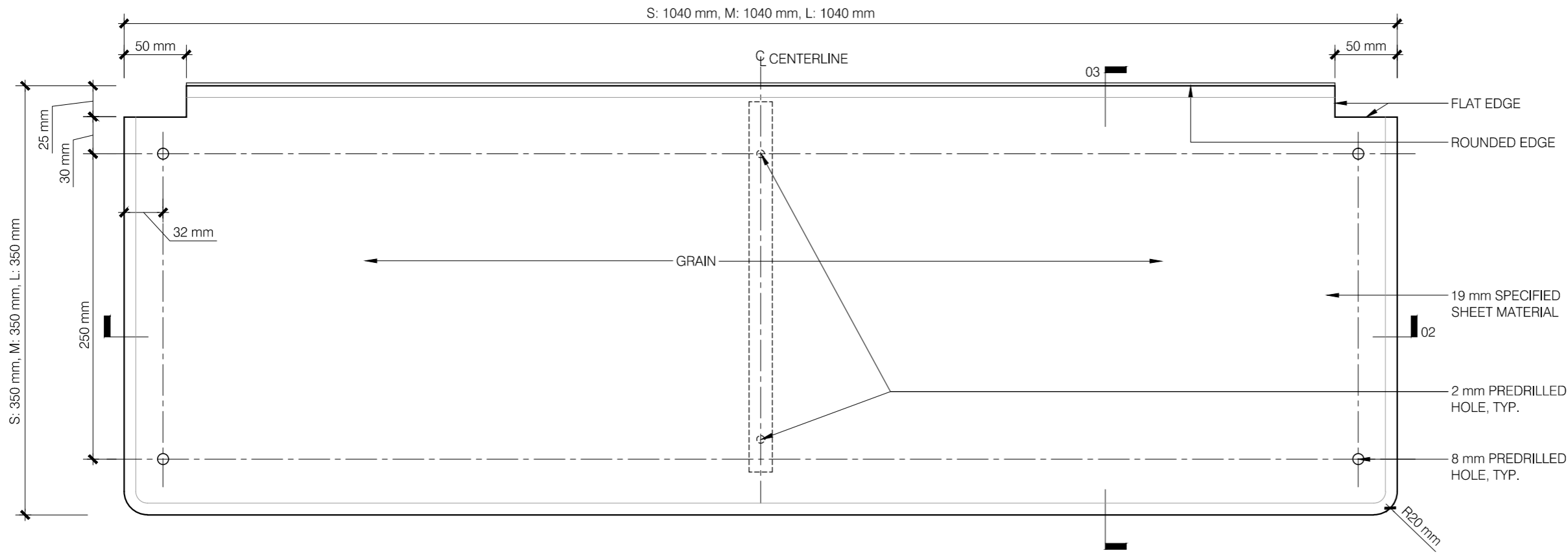
01 SHELF PLAN 1:4 SCALE
