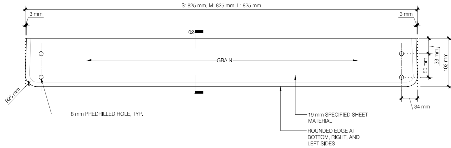
01 BENCH KNEE PANEL ELEVATION 1/4 SCALE
