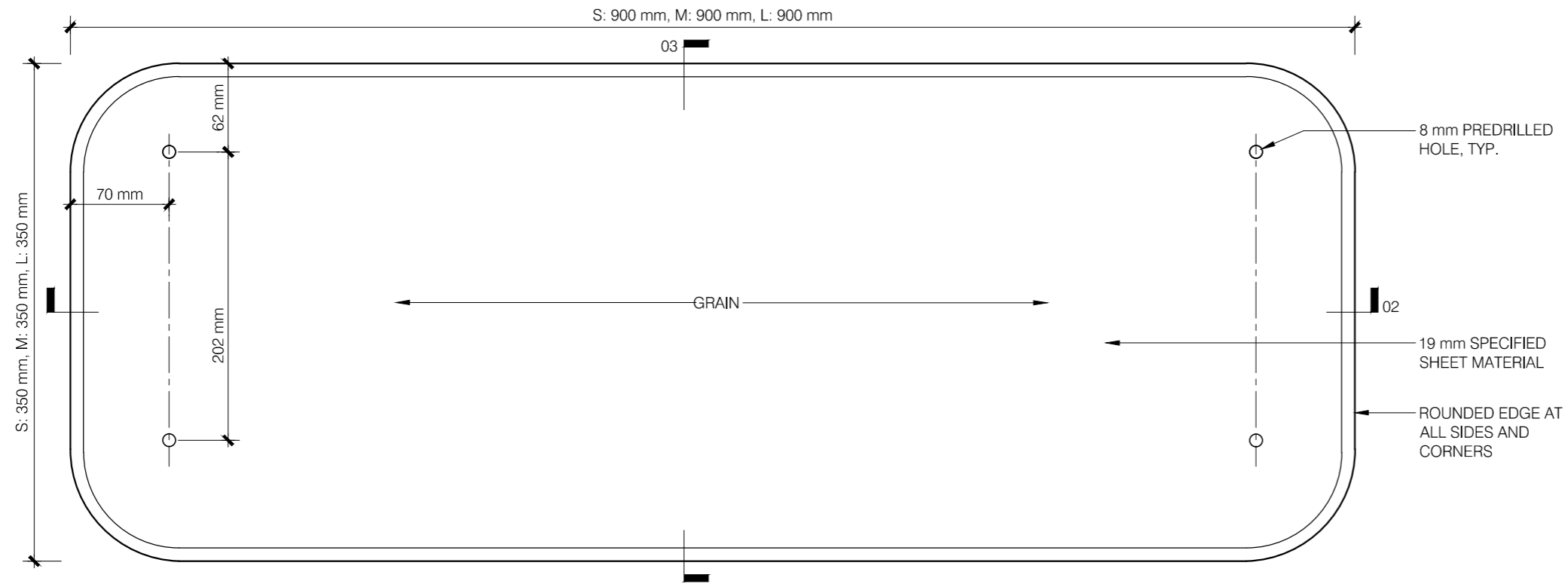
01 BENCH SEAT PLAN 1:4 SCALE
