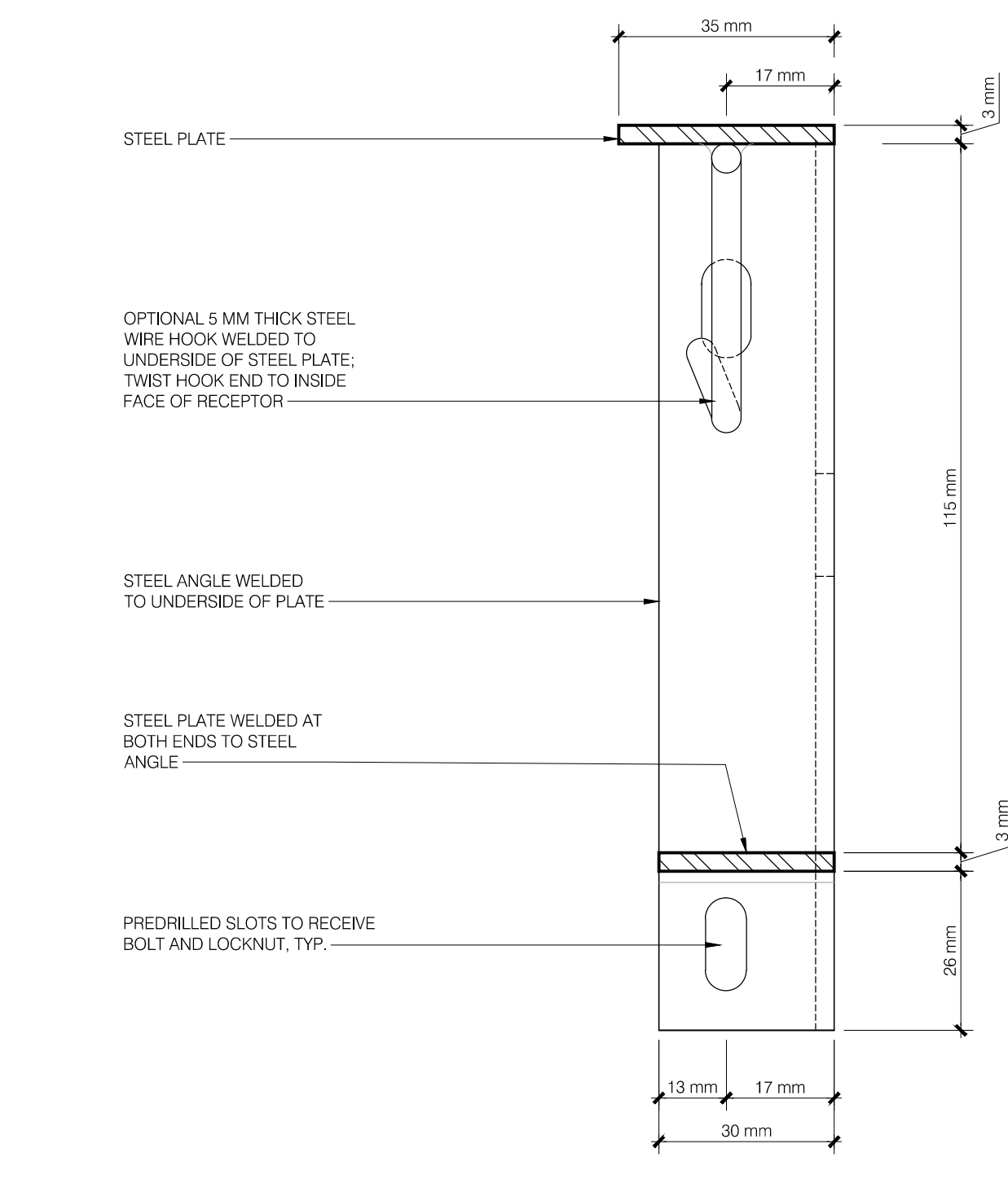
04 DESK LEFT SIDE RECEPTOR SECTION 1:1 SCALE
