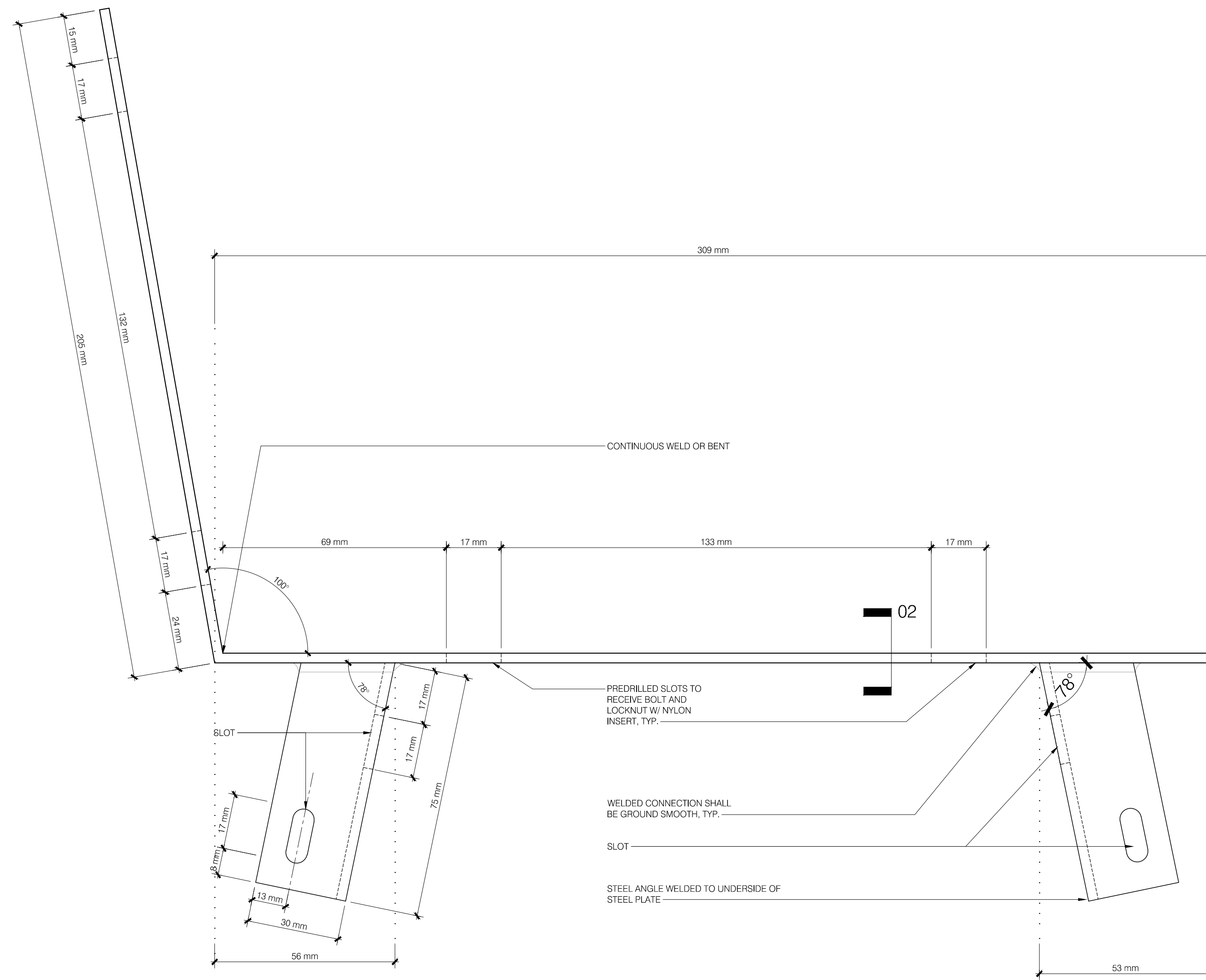
01 CHAIR RIGHT SIDE RECEPTOR ELEVATION 1:1 SCALE
