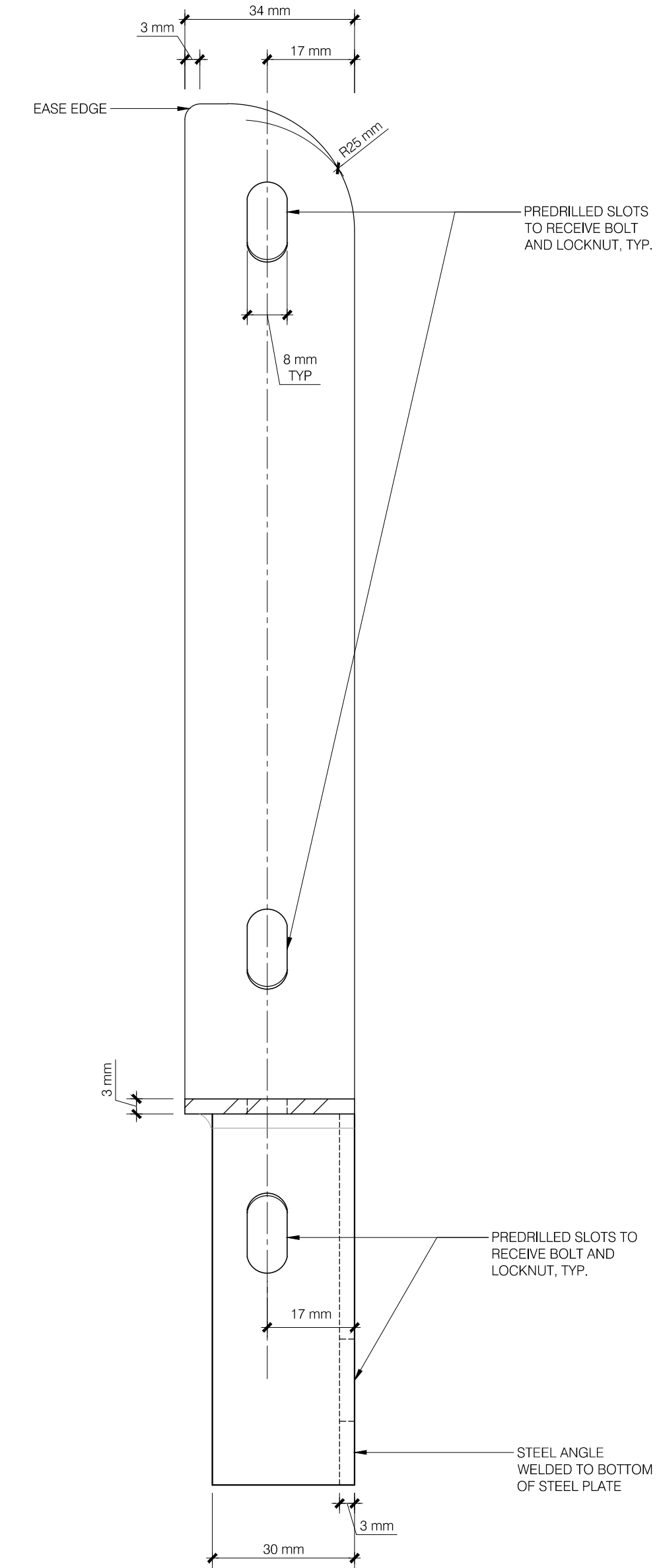
02 CHAIR LEFT SIDE RECEPTOR SECTION 1:1 SCALE
