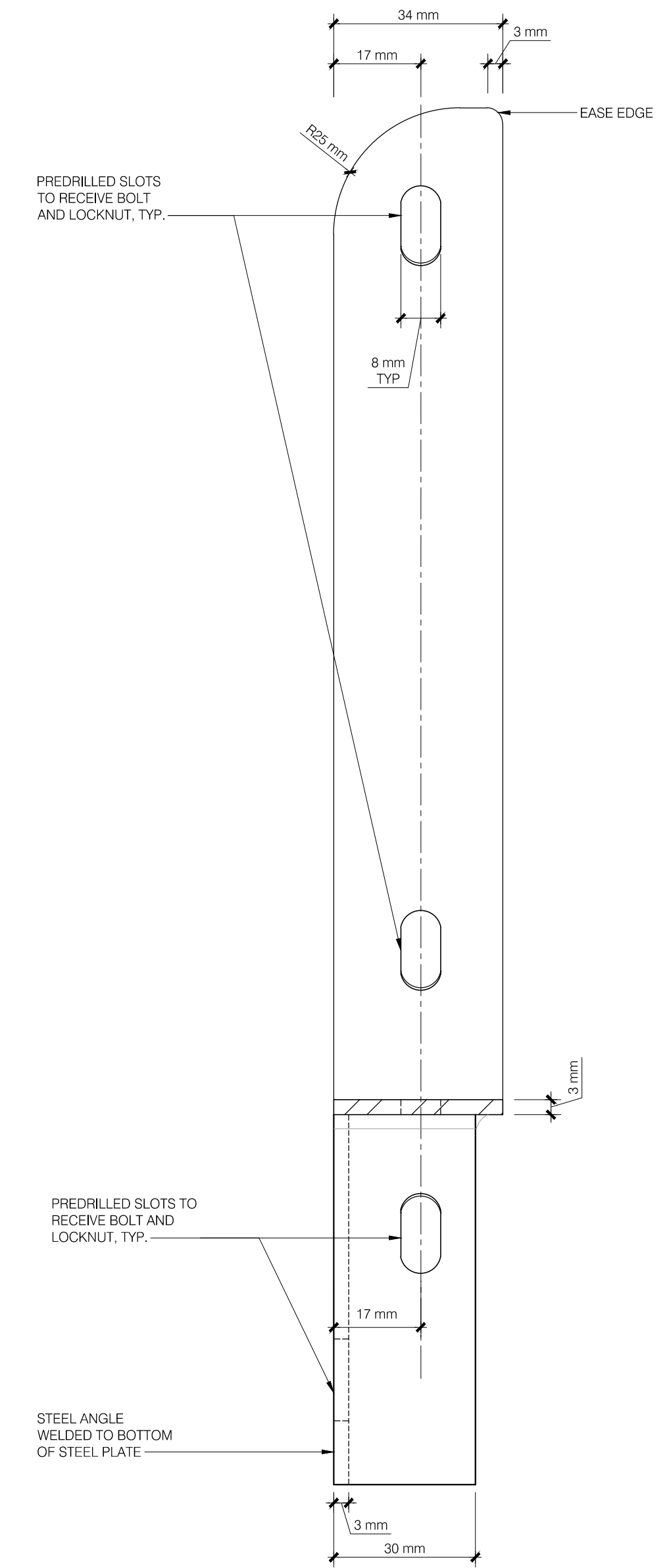
02 CHAIR RIGHT SIDE RECEPTOR SECTION 1:1 SCALE
